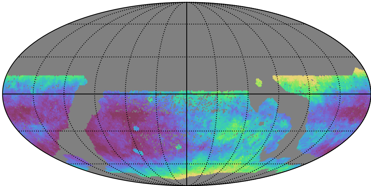
smc_lmc_v3.3_10yrs WFD r band: Median seeingEff
