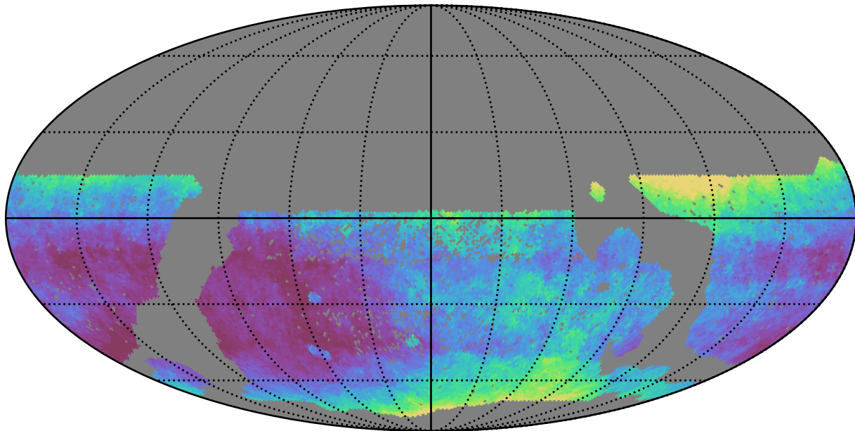
smc_lmc_v3.3_10yrs WFD i band: Median seeingEff
