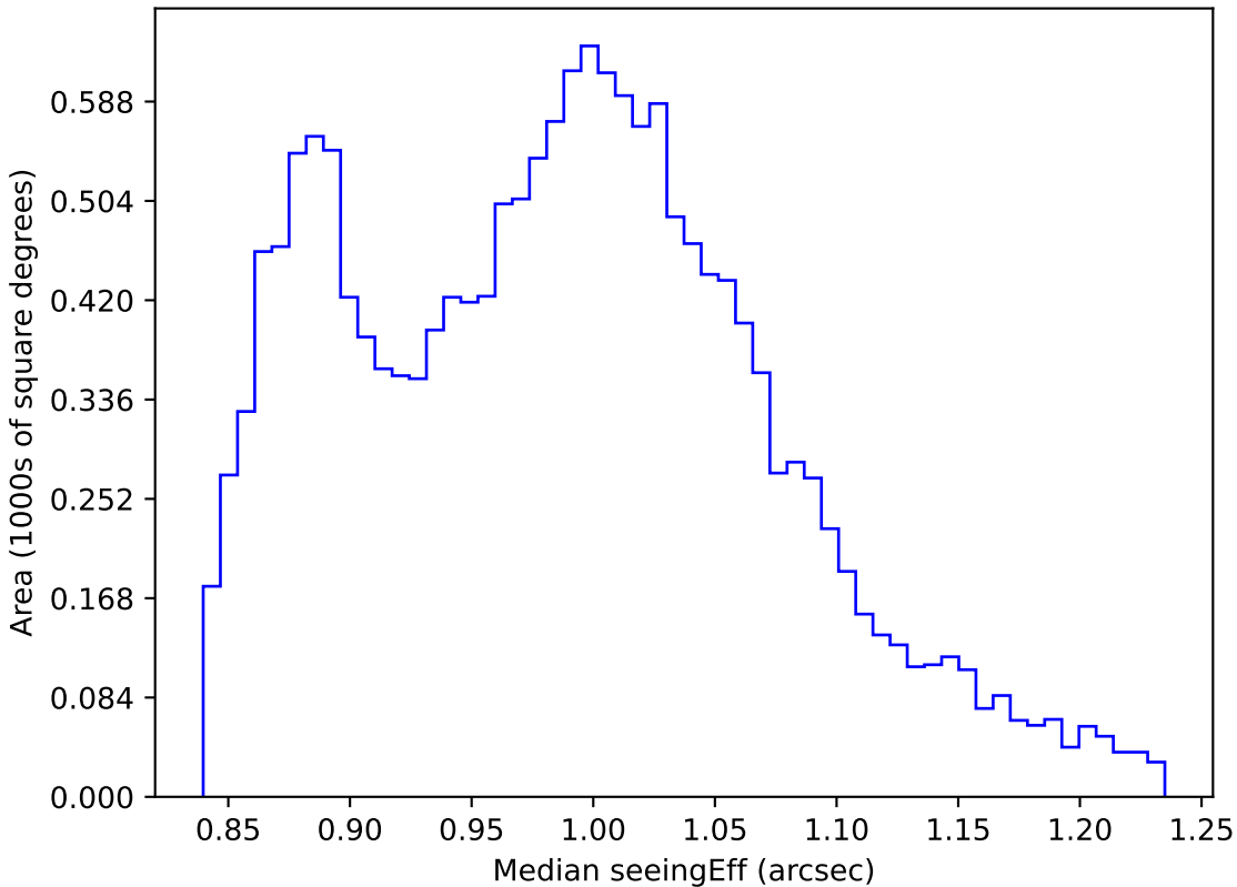
smc_lmc_v3.3_10yrs WFD i band: Median seeingEff
