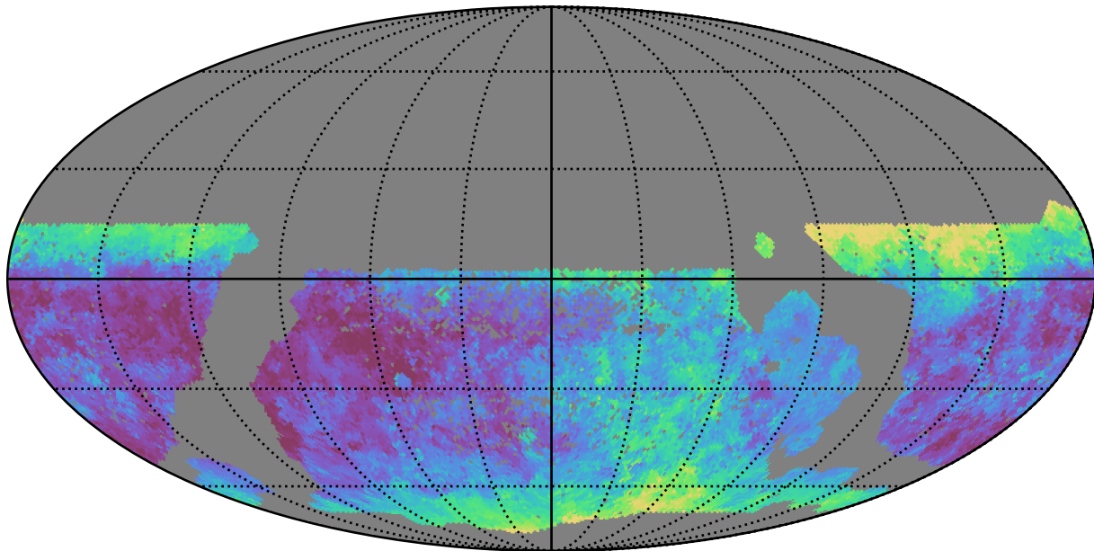
smc_lmc_v3.3_10yrs WFD g band: Median seeingEff
