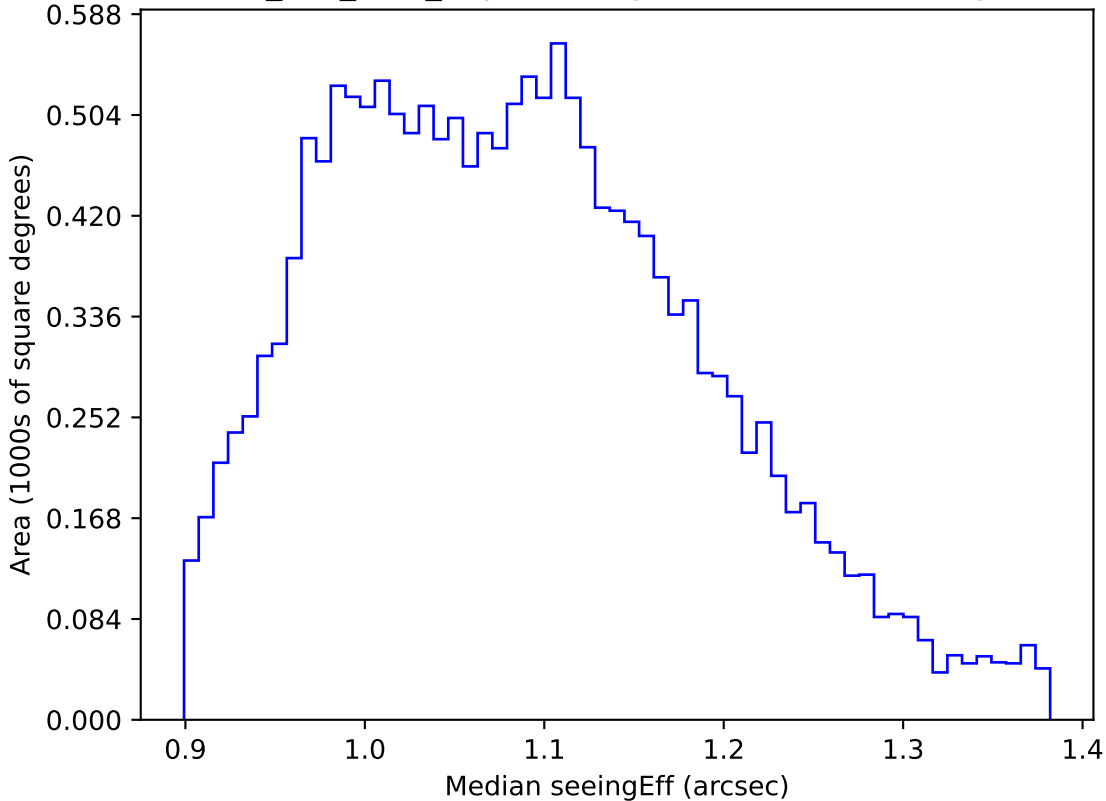
smc_lmc_v3.3_10yrs WFD g band: Median seeingEff
