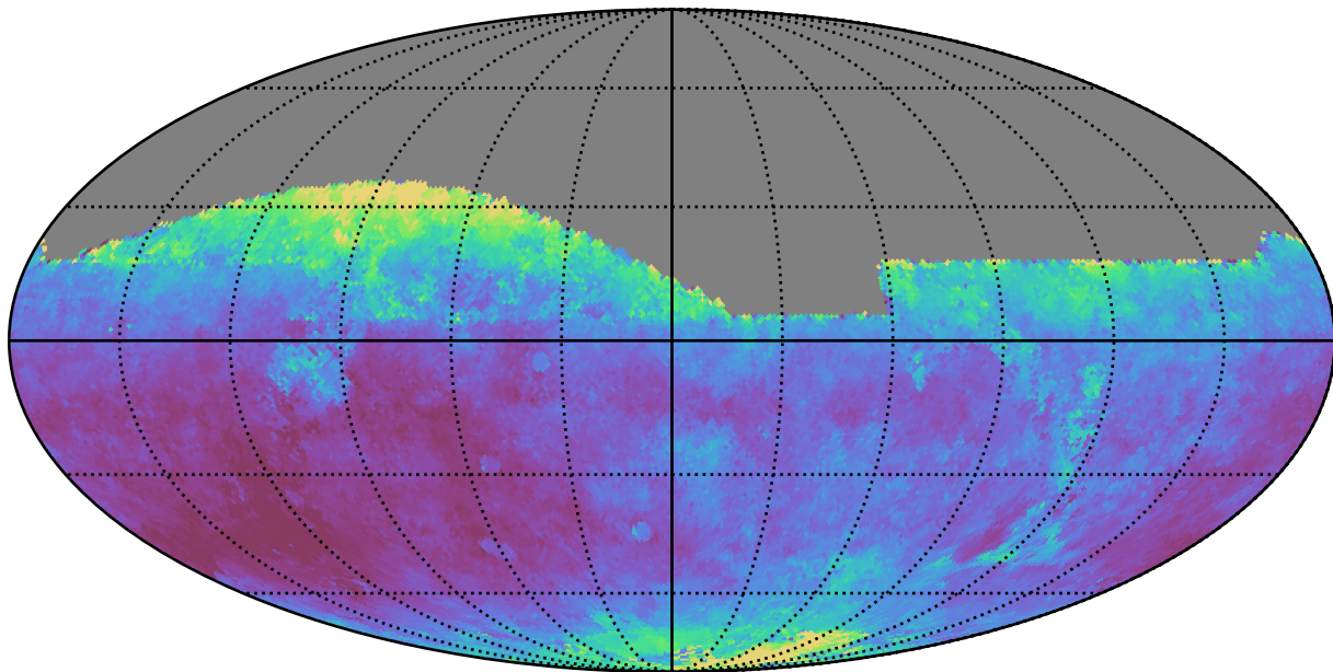
smc_lmc_v3.3_10yrs All sky z band: Median seeingEff
