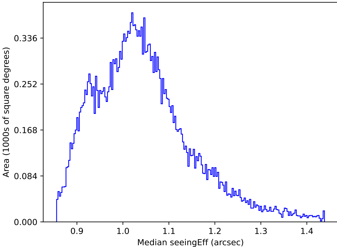
smc_lmc_v3.3_10yrs All sky z band: Median seeingEff
