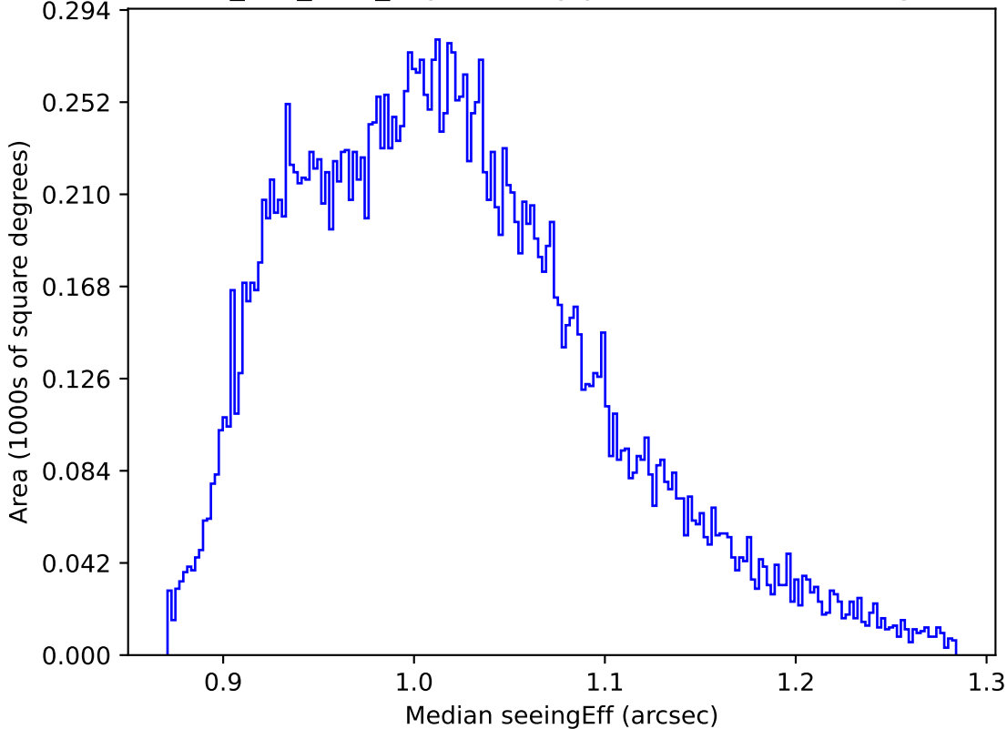
smc_lmc_v3.3_10yrs All sky y band: Median seeingEff
