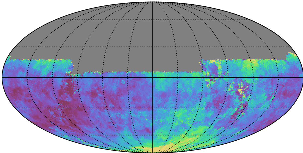
smc_lmc_v3.3_10yrs All sky u band: Median seeingEff
