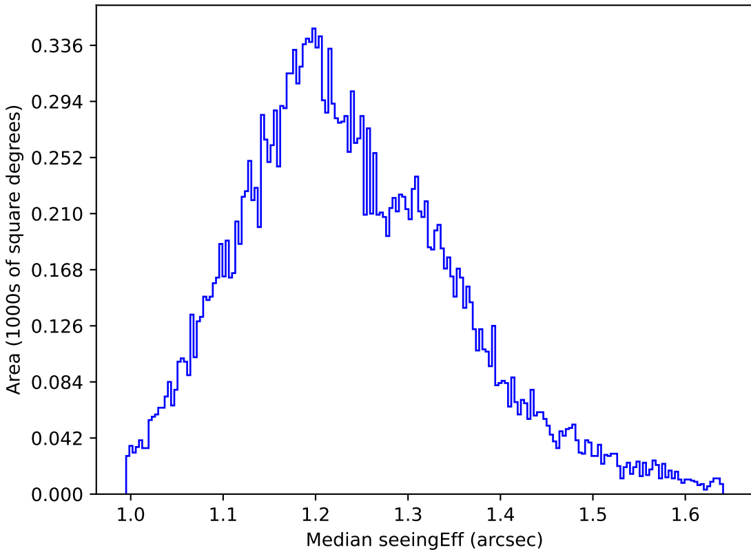
smc_lmc_v3.3_10yrs All sky u band: Median seeingEff
