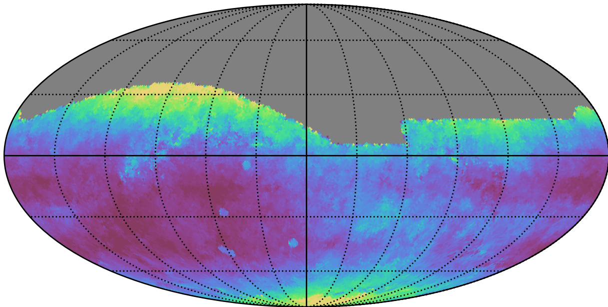
smc_lmc_v3.3_10yrs All sky r band: Median seeingEff
