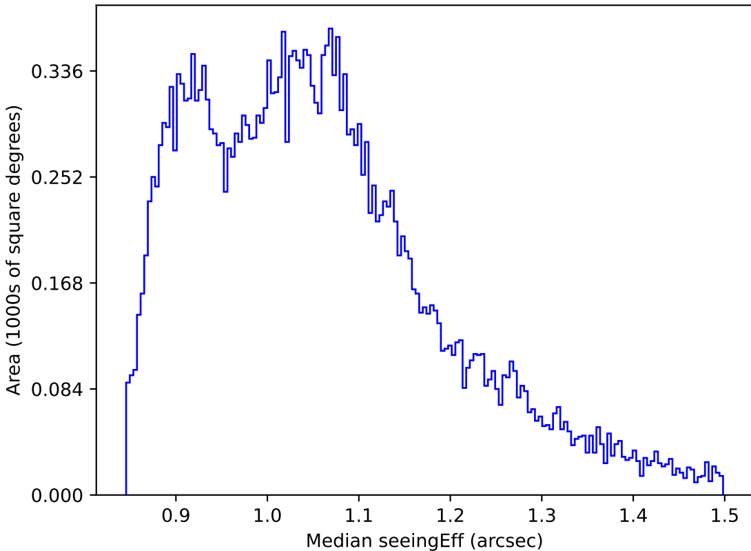
smc_lmc_v3.3_10yrs All sky r band: Median seeingEff
