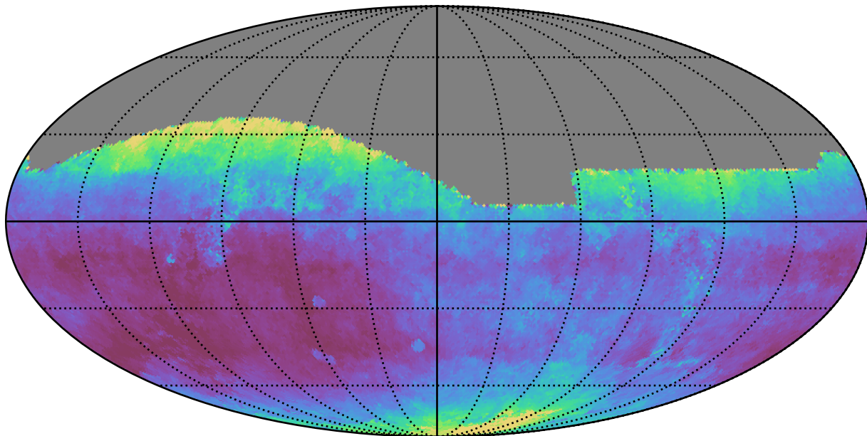
smc_lmc_v3.3_10yrs All sky i band: Median seeingEff
