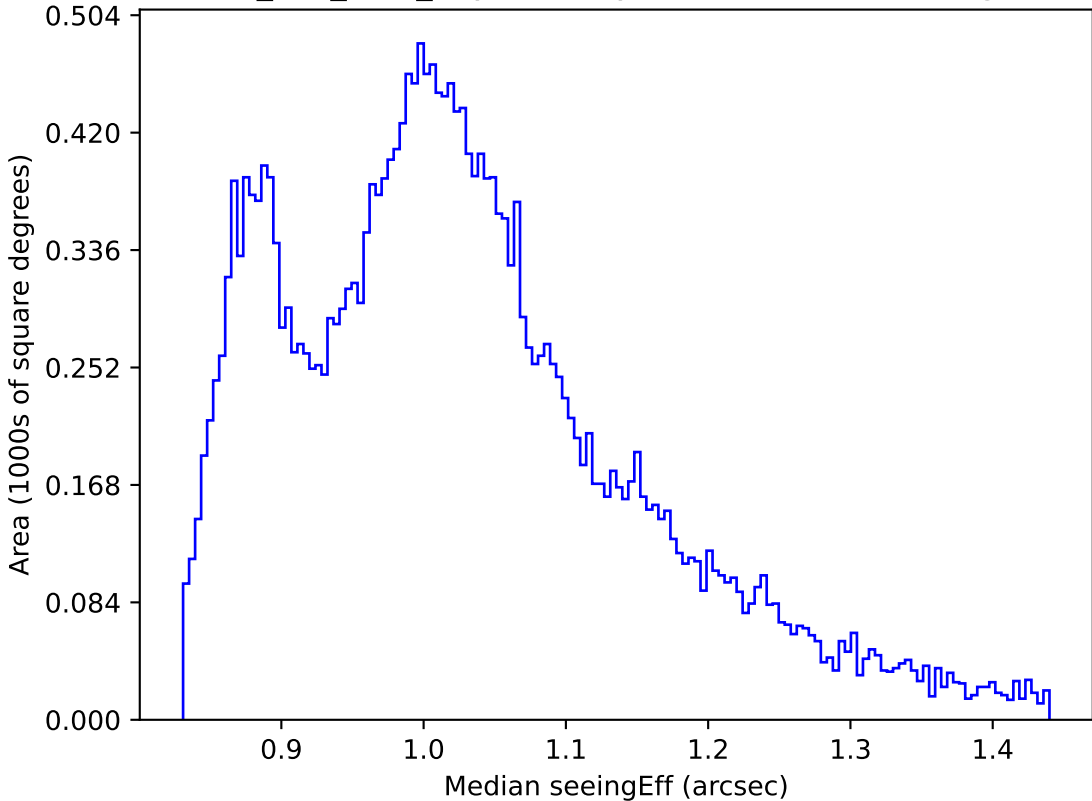
smc_lmc_v3.3_10yrs All sky i band: Median seeingEff
