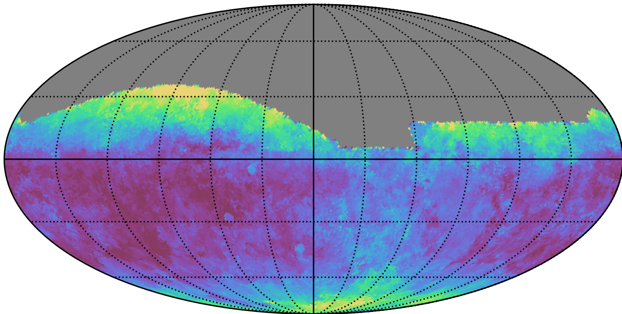
smc_lmc_v3.3_10yrs All sky g band: Median seeingEff
