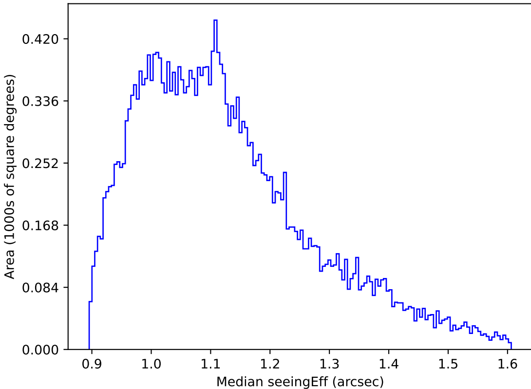
smc_lmc_v3.3_10yrs All sky g band: Median seeingEff
