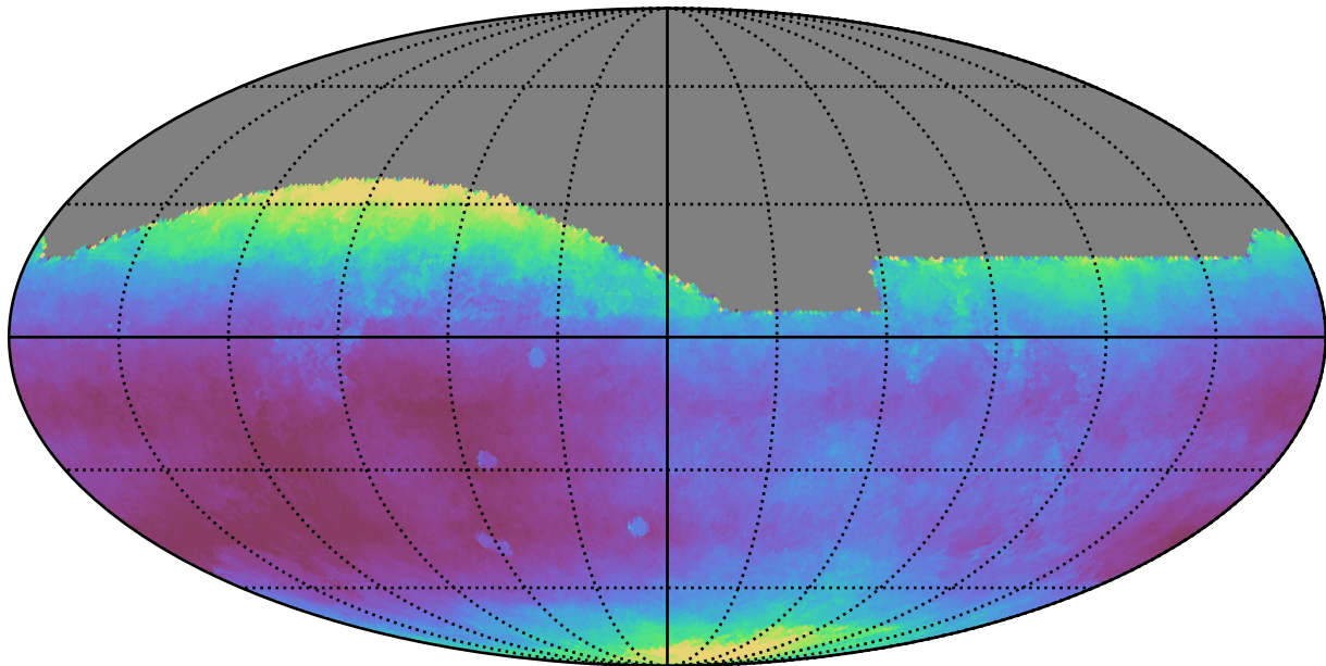
smc_lmc_v3.3_10yrs All sky all bands: Median seeingEff
