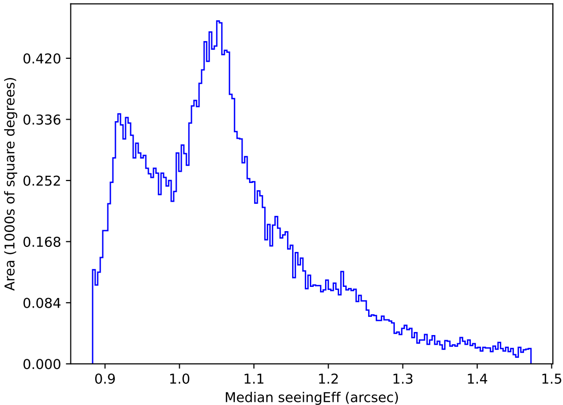
smc_lmc_v3.3_10yrs All sky all bands: Median seeingEff
