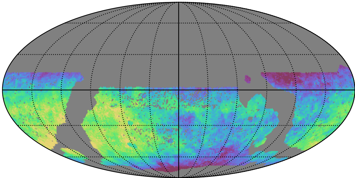
smc_lmc_v3.3_10yrs WFD z band: Median saturation_mag
