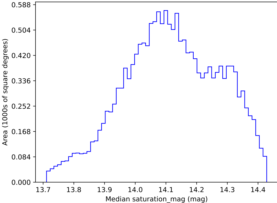
smc_lmc_v3.3_10yrs WFD z band: Median saturation_mag
