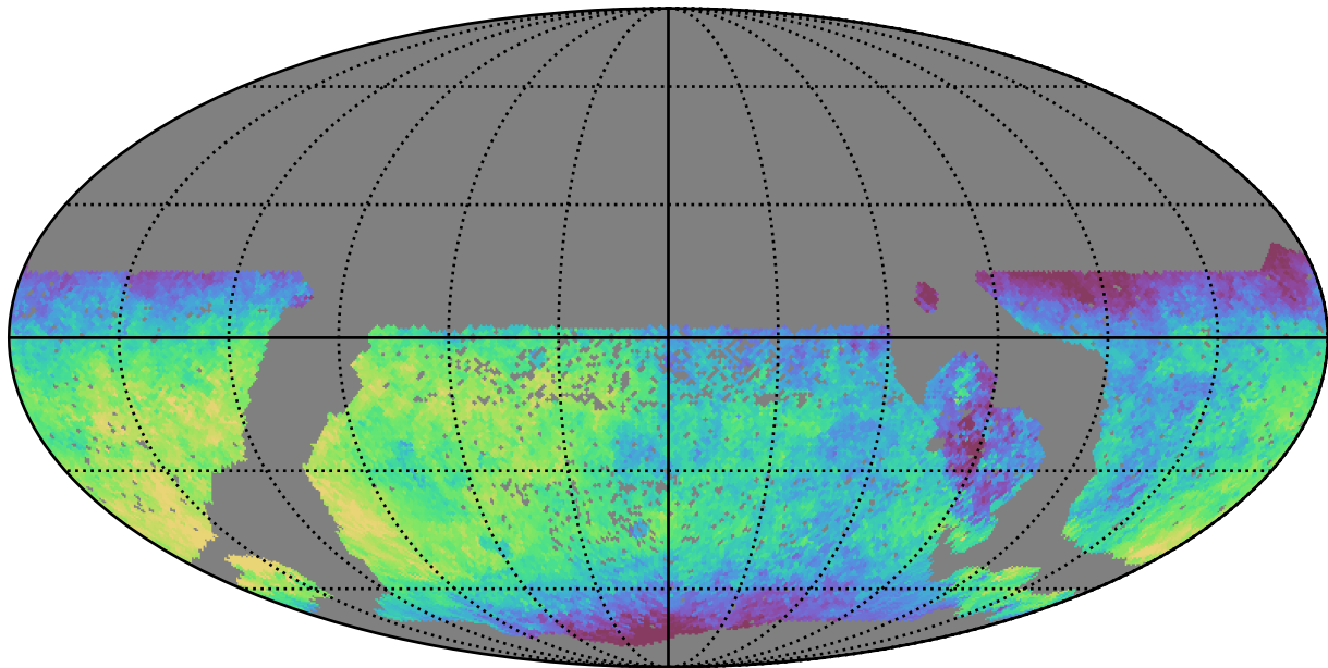
smc_lmc_v3.3_10yrs WFD y band: Median saturation_mag
