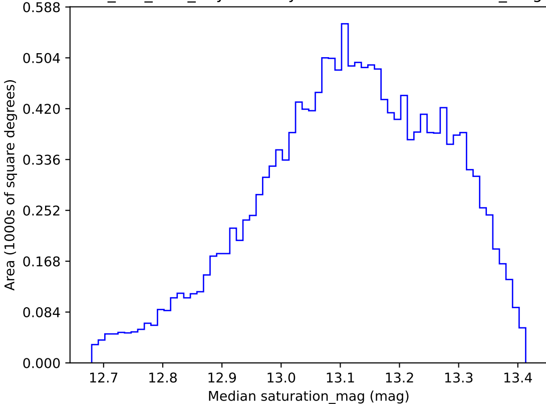
smc_lmc_v3.3_10yrs WFD y band: Median saturation_mag
