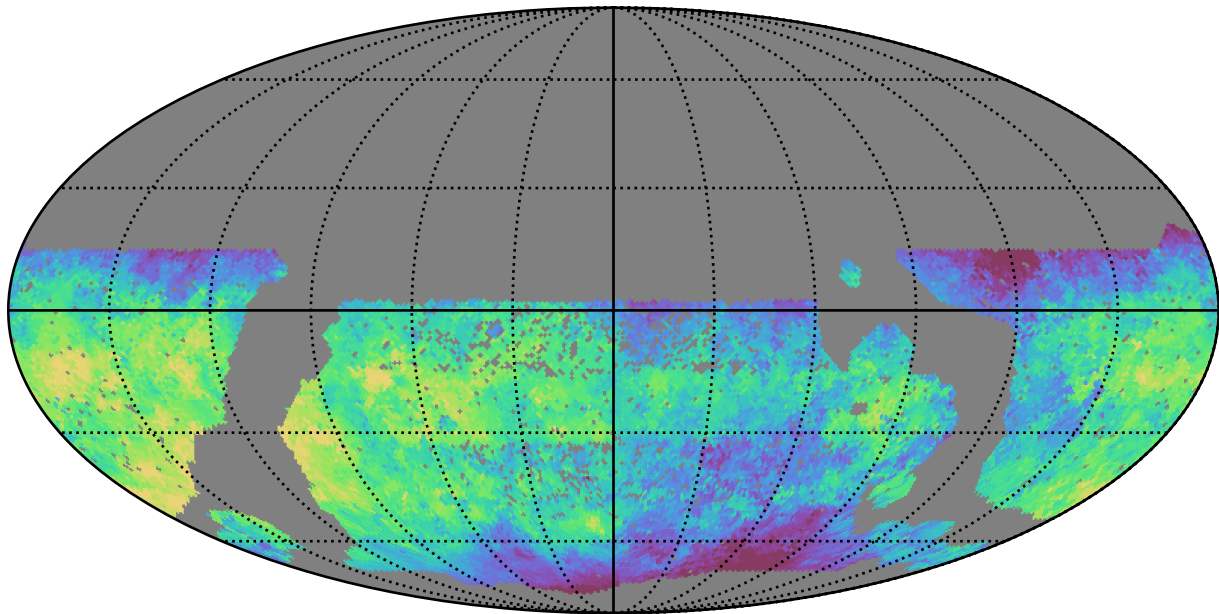
smc_lmc_v3.3_10yrs WFD u band: Median saturation_mag
