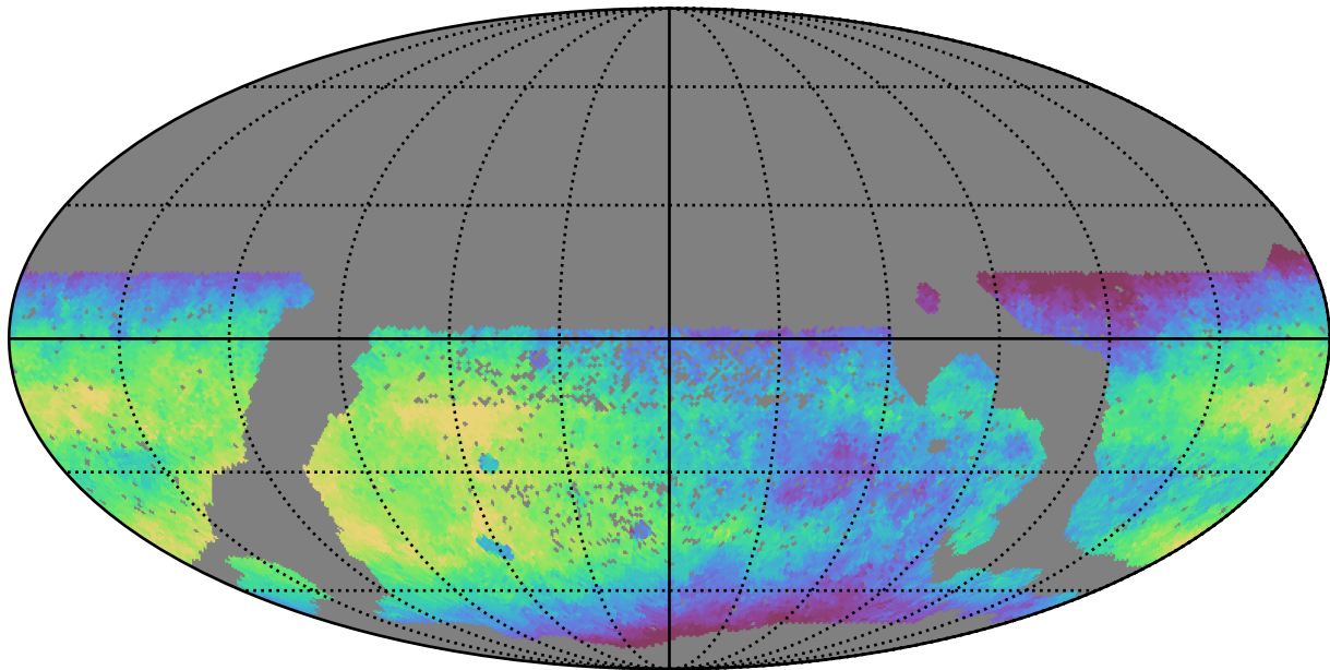
smc_lmc_v3.3_10yrs WFD r band: Median saturation_mag
