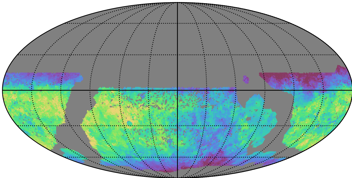
smc_lmc_v3.3_10yrs WFD g band: Median saturation_mag
