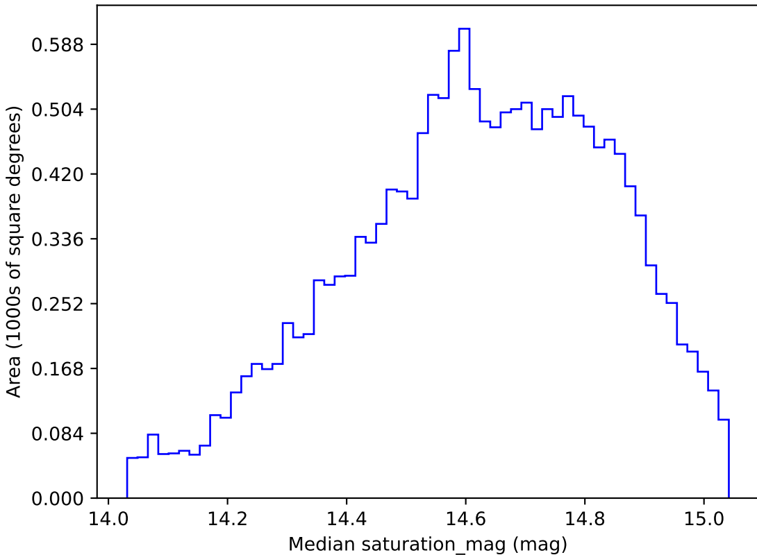
smc_lmc_v3.3_10yrs WFD g band: Median saturation_mag
