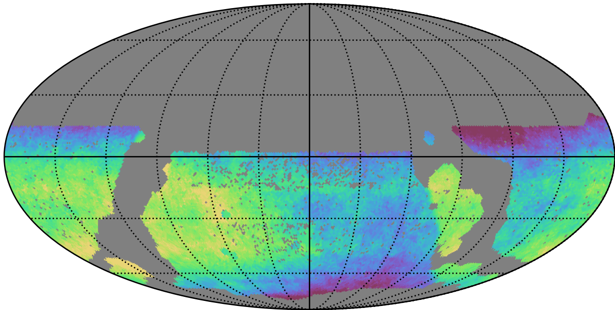
smc_lmc_v3.3_10yrs WFD all bands: Median saturation_mag
