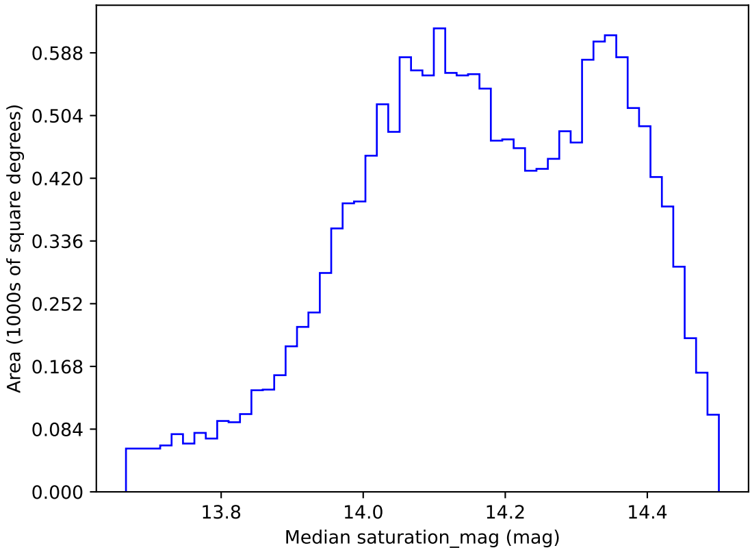
smc_lmc_v3.3_10yrs WFD all bands: Median saturation_mag
