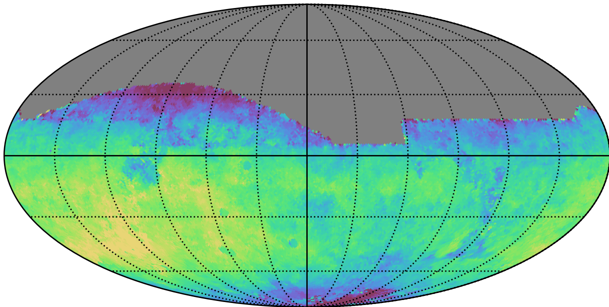
smc_lmc_v3.3_10yrs All sky z band: Median saturation_mag
