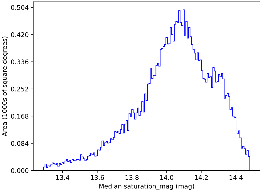
smc_lmc_v3.3_10yrs All sky z band: Median saturation_mag
