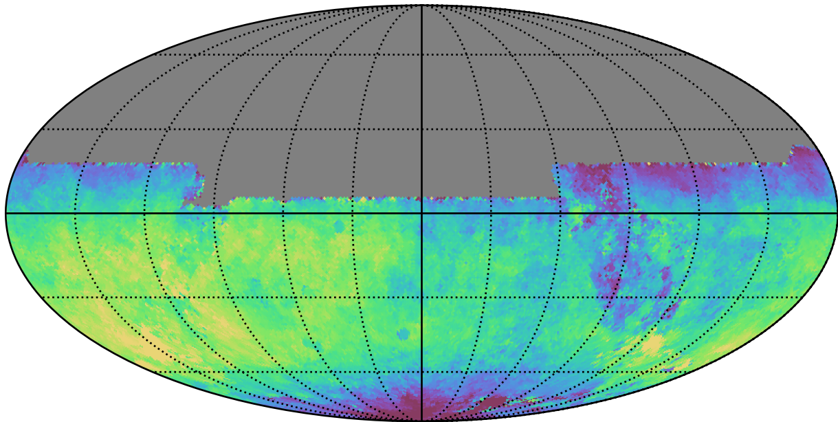
smc_lmc_v3.3_10yrs All sky y band: Median saturation_mag
