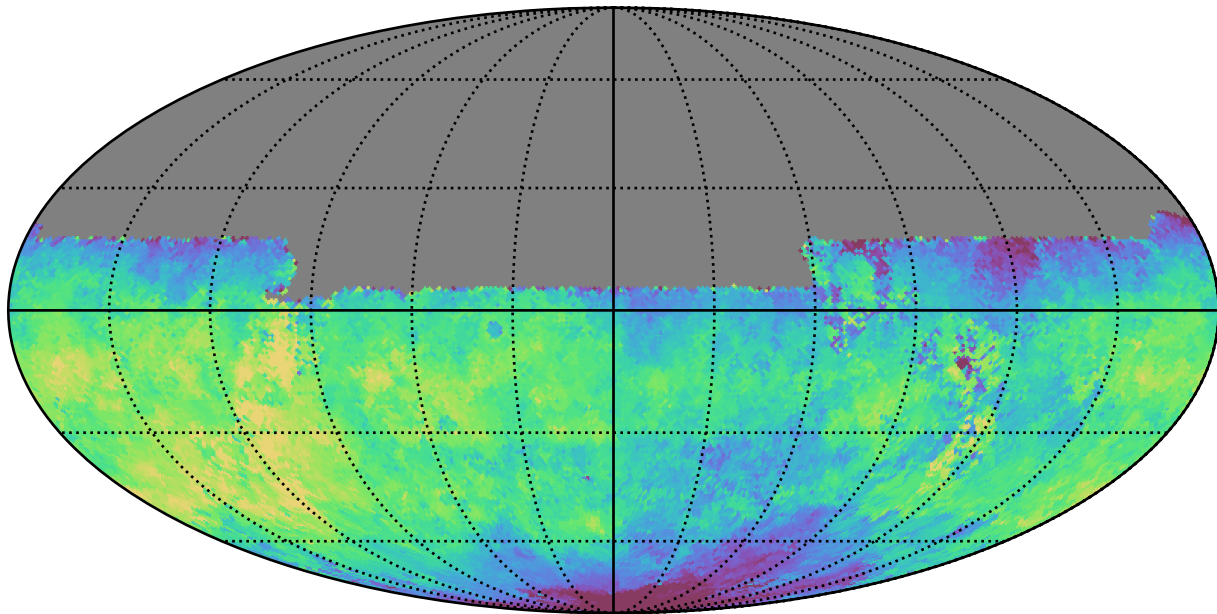
smc_lmc_v3.3_10yrs All sky u band: Median saturation_mag
