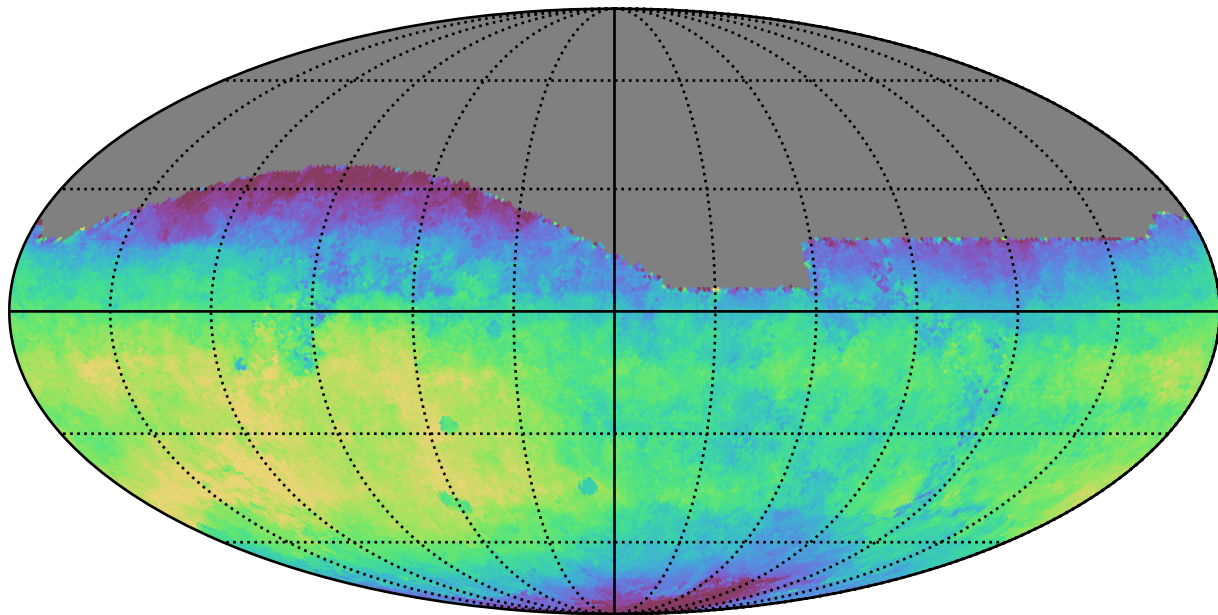
smc_lmc_v3.3_10yrs All sky i band: Median saturation_mag
