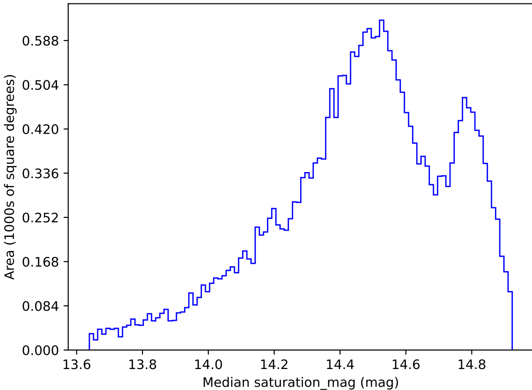
smc_lmc_v3.3_10yrs All sky i band: Median saturation_mag
