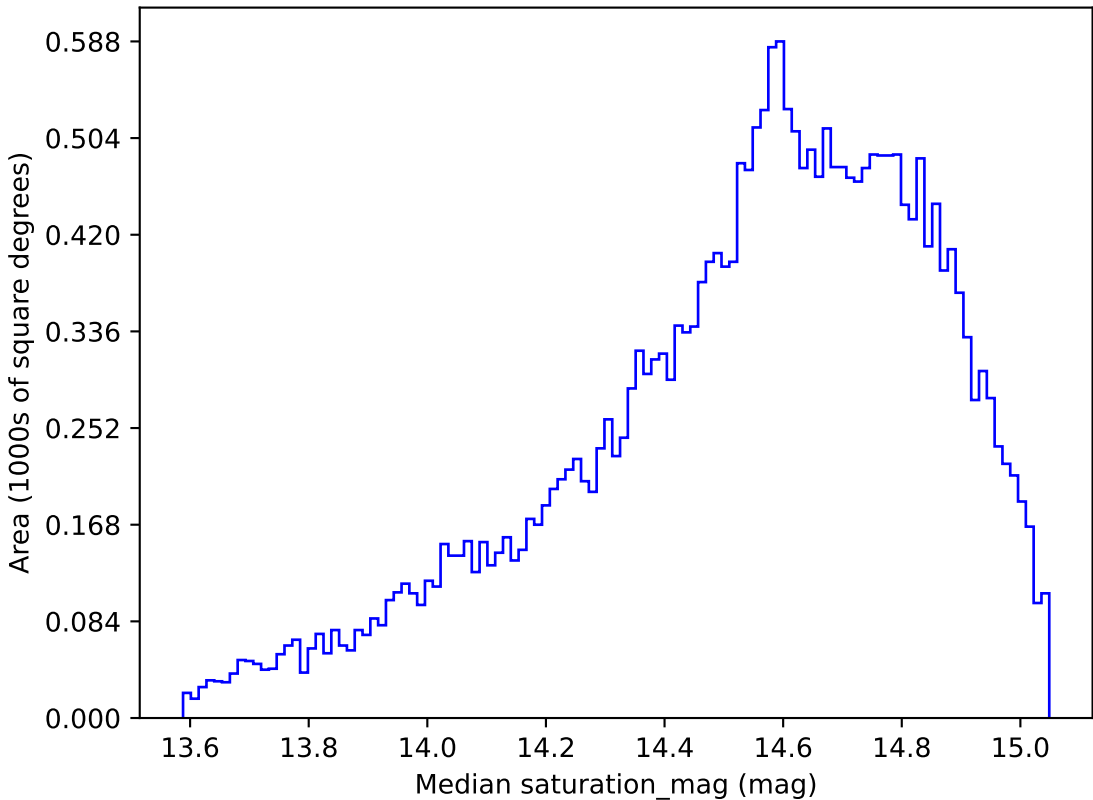
smc_lmc_v3.3_10yrs All sky g band: Median saturation_mag
