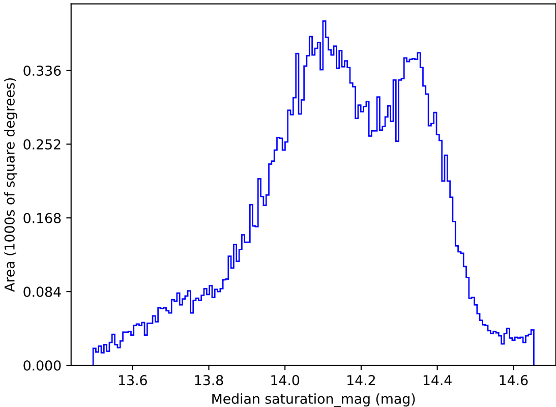
smc_lmc_v3.3_10yrs All sky all bands: Median saturation_mag
