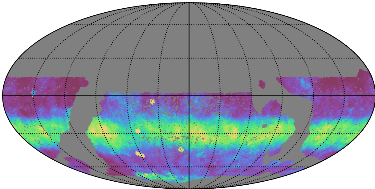
smc_lmc_v3.3_10yrs WFD z band: Median normairmass
