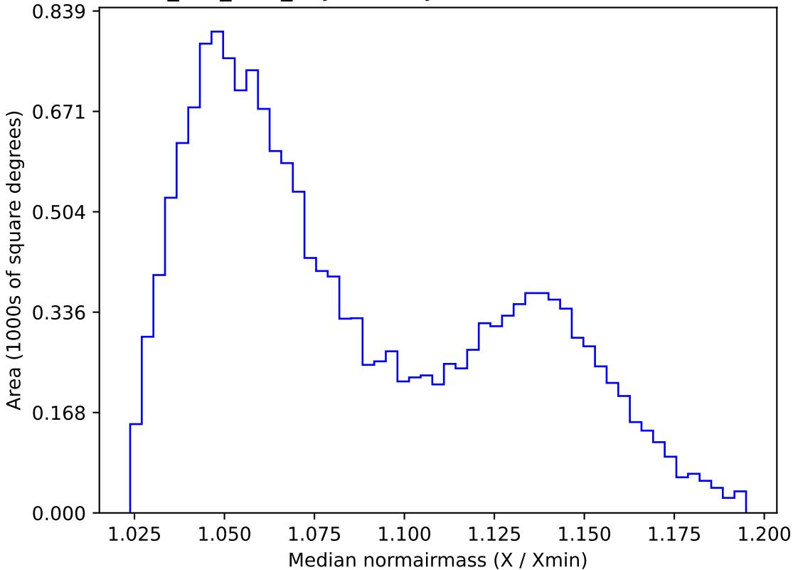
smc_lmc_v3.3_10yrs WFD y band: Median normairmass
