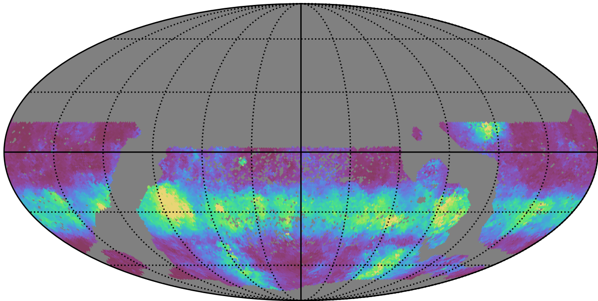
smc_lmc_v3.3_10yrs WFD u band: Median normairmass
