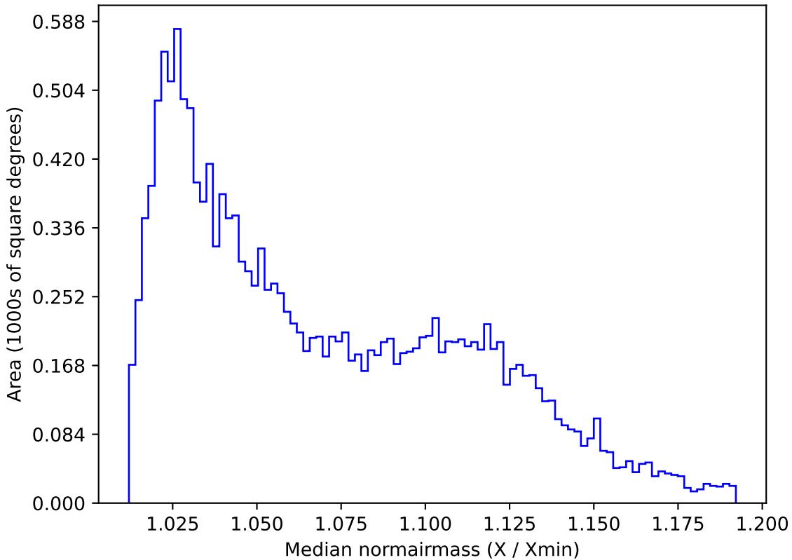
smc_lmc_v3.3_10yrs WFD u band: Median normairmass
