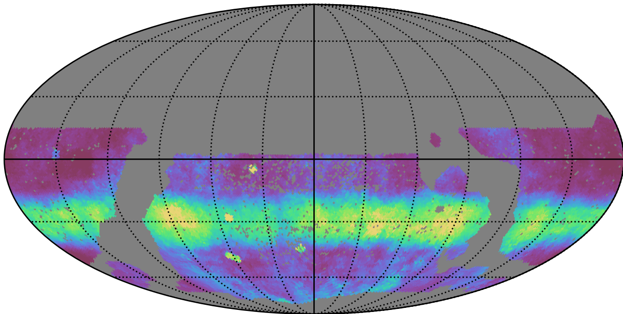
smc_lmc_v3.3_10yrs WFD r band: Median normairmass
