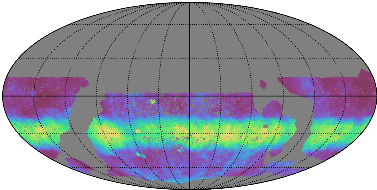
smc_lmc_v3.3_10yrs WFD i band: Median normairmass
