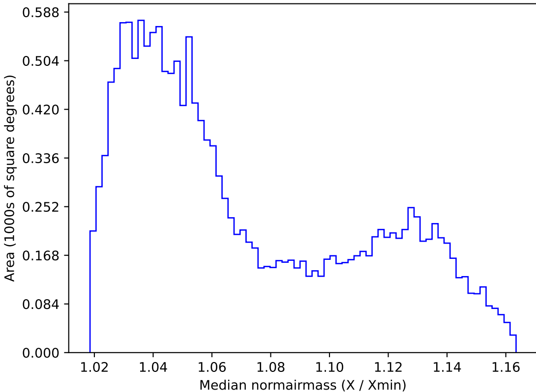
smc_lmc_v3.3_10yrs WFD i band: Median normairmass
