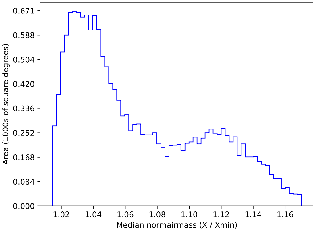
smc_lmc_v3.3_10yrs WFD g band: Median normairmass
