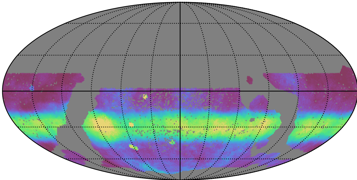
smc_lmc_v3.3_10yrs WFD all bands: Median normairmass
