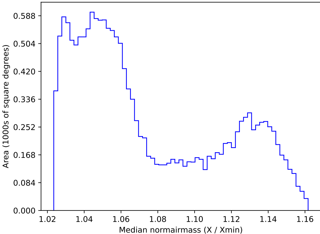
smc_lmc_v3.3_10yrs WFD all bands: Median normairmass
