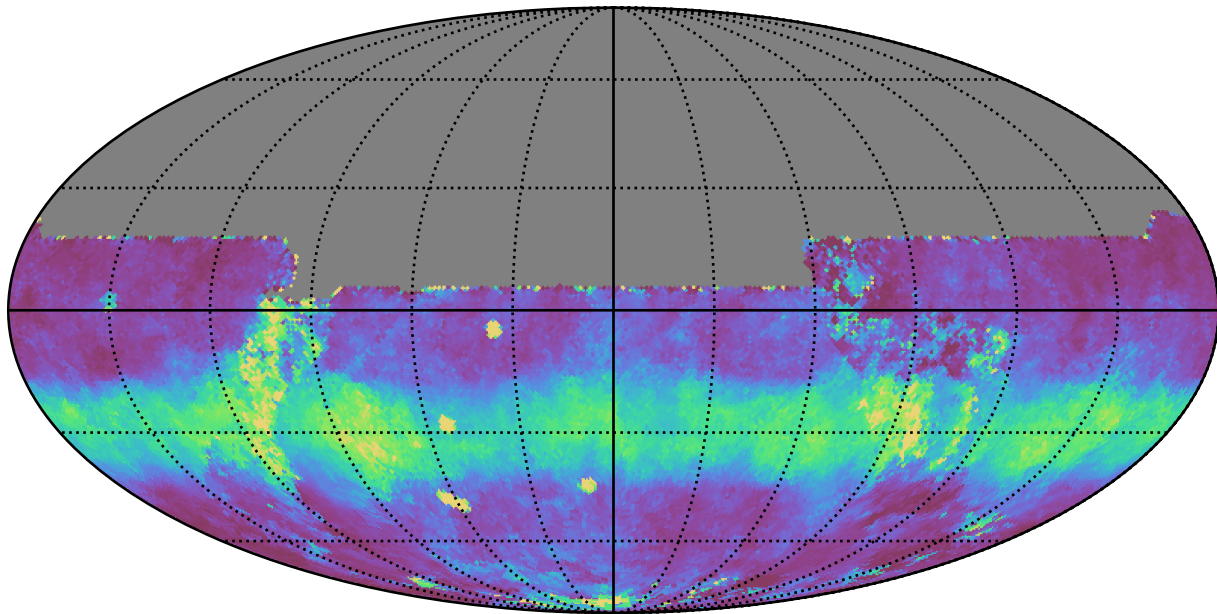
smc_lmc_v3.3_10yrs All sky y band: Median normairmass
