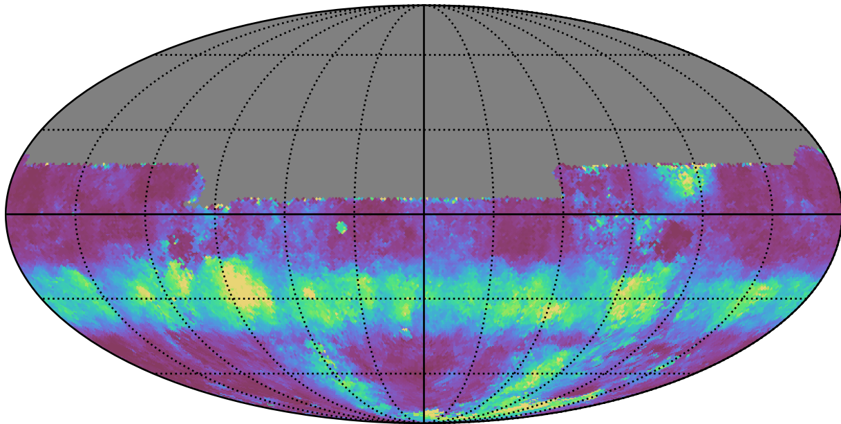
smc_lmc_v3.3_10yrs All sky u band: Median normairmass
