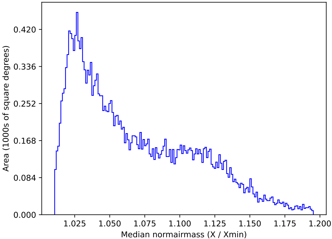
smc_lmc_v3.3_10yrs All sky u band: Median normairmass
