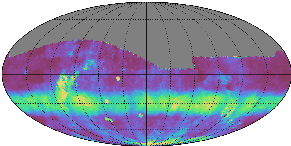
smc_lmc_v3.3_10yrs All sky r band: Median normairmass
